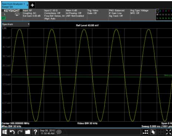
Figure 10-8 AM Signal Measured in the Time Domain
