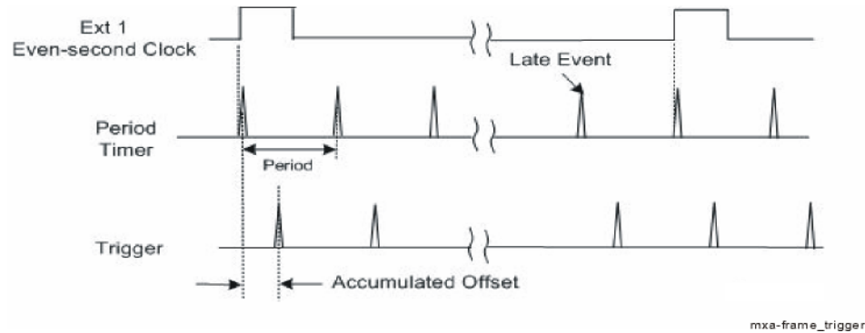
Figure 12-2 Frame Triggering
