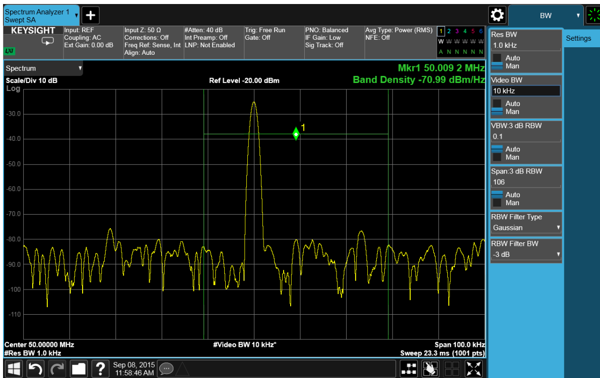
Figure 7-5 Band/Interval Density Measurement
