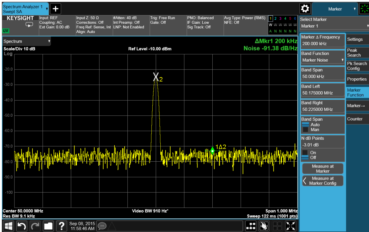
Figure 7-1 Measuring Signal-to-Noise
