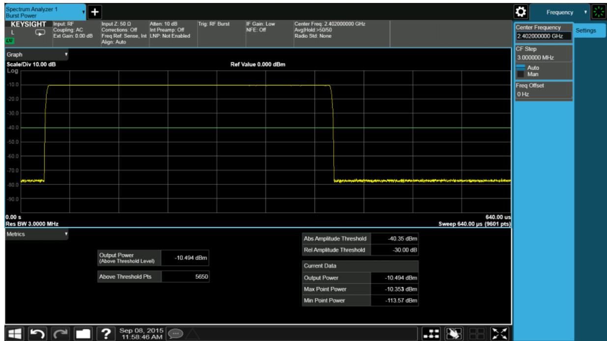
Figure 9-12 Normal Screen Display of Burst Power Measurement Results
