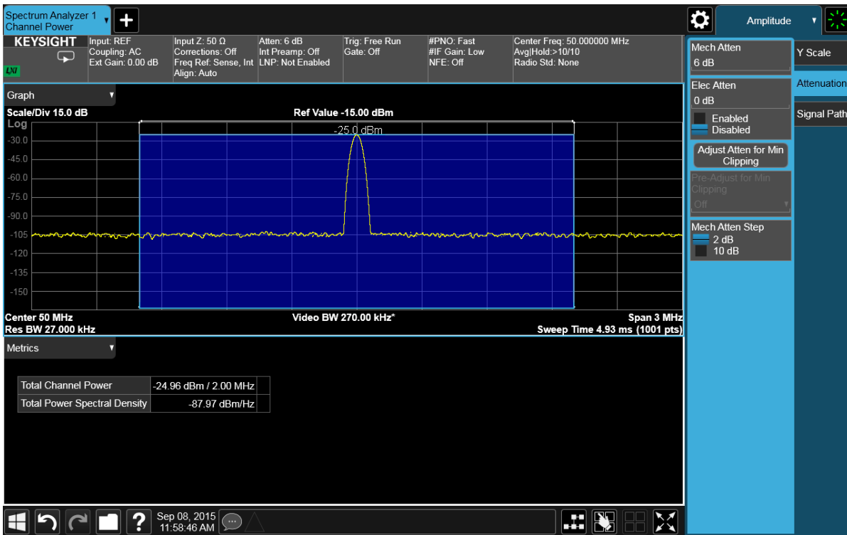
Figure 7-7 Measuring Channel Power
