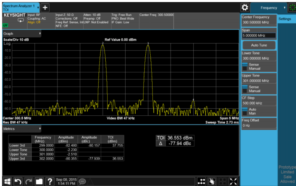
Figure 6-7 TOI Measurement
