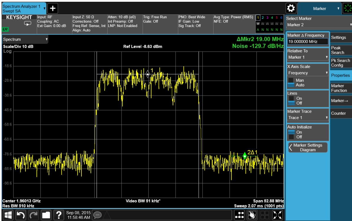
Figure 7-10 Signal-to-Noise Measurement
