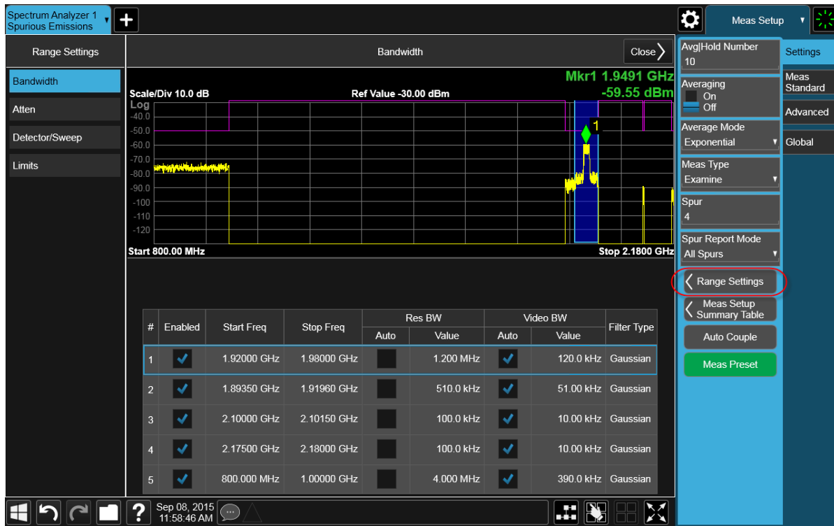
Figure 9-18 Spurious Emission Measurement - Range Settings
