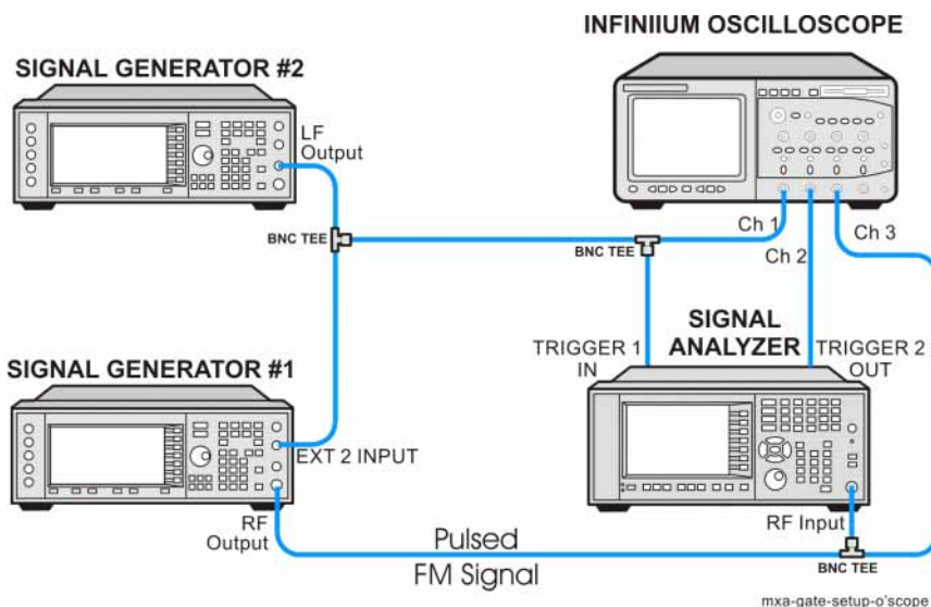
Figure 8-4 Instrument Connection Diagram with Oscilloscope
